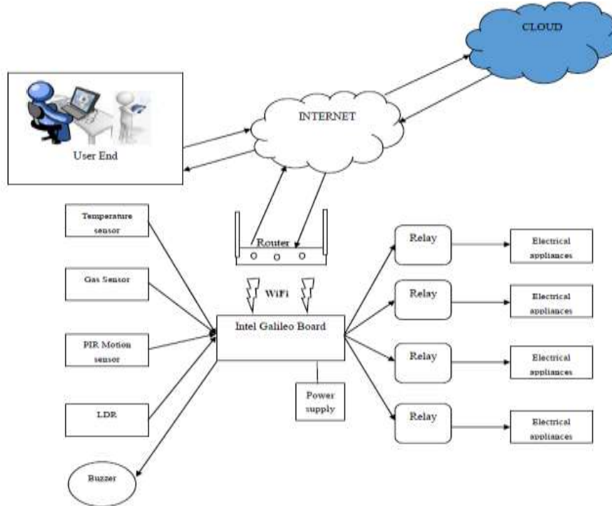
Fig.1: Architecture [1]
